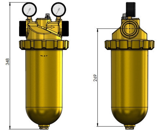
Filter 1 1/4" DN32
